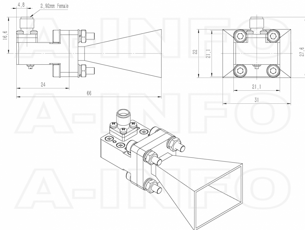
2.92mm-Female Output (P/N: LB-34-15-C-KF)
