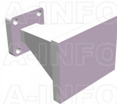
LB-34-15-ASPO Standard Gain Horn Antenna 22-33GHz 15dB Gain Rectangular Waveguide Interface
